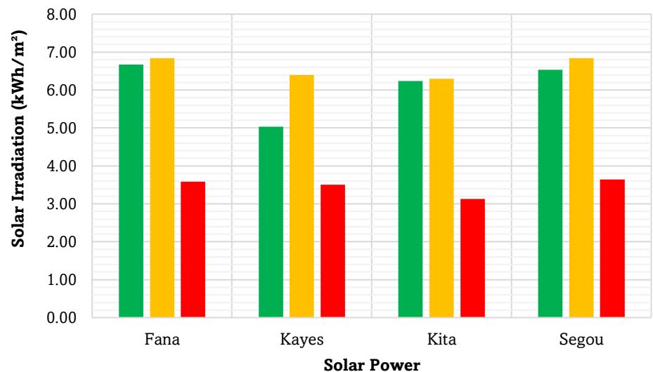
Figure 6 . The comparative histogram of the different solar irradiations of the four cities.
