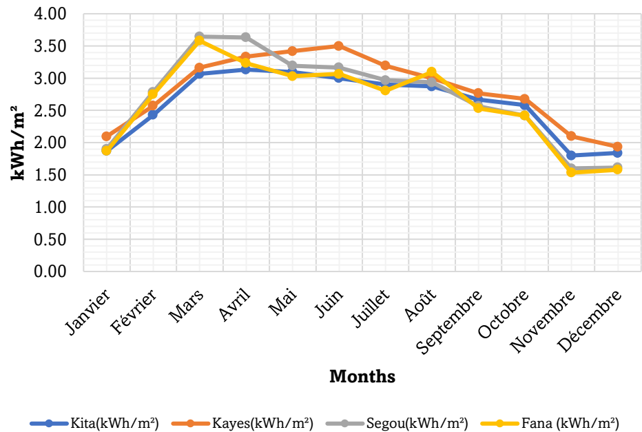
Figure 4 . The different horizontal diffuse irradiations of the four cities.
