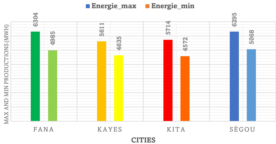
Figure 9 . The maximum and minimum production of the different cities.
