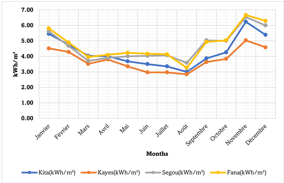
Figure 5. The different diffuse normal irradiations of the four cities.
