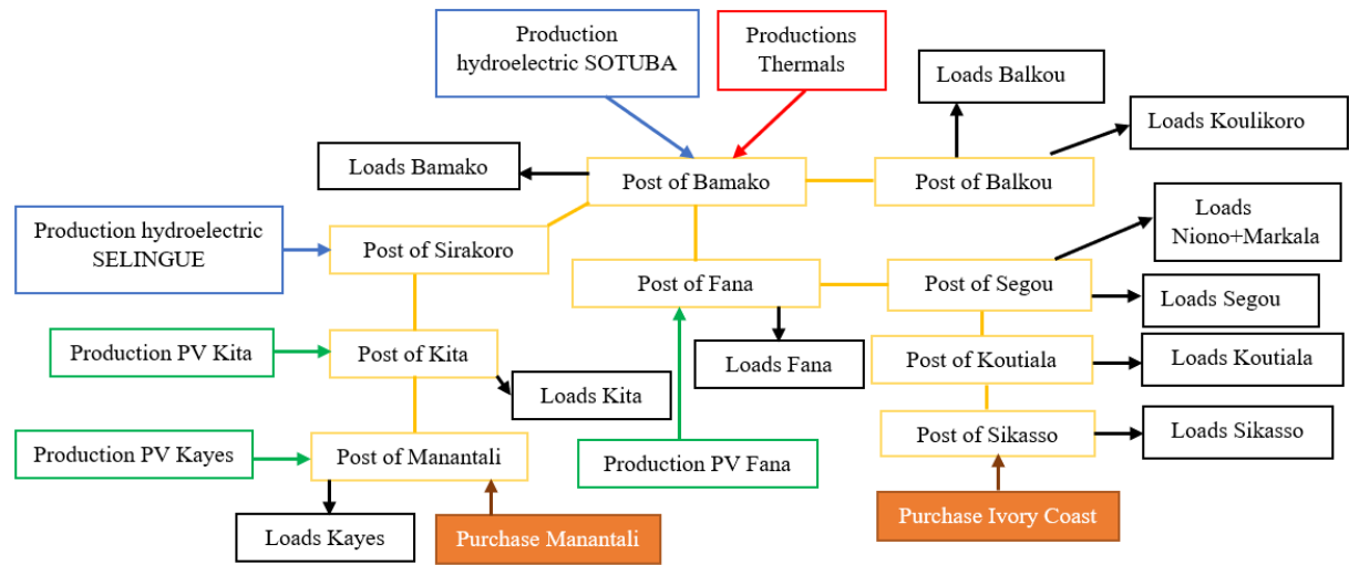
Figure 2 . Mali electricity supply interconnection network.
