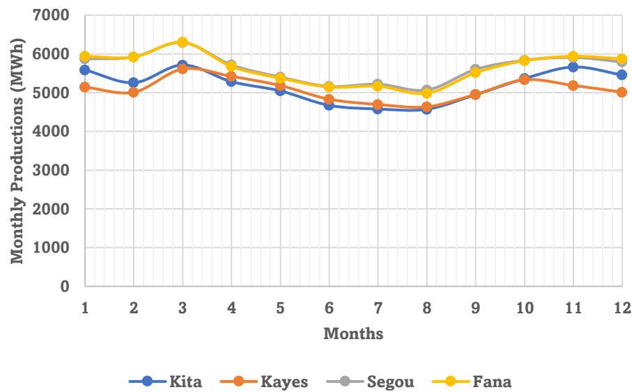
Figure 10. The curve of the various monthly productions during the twelve (12) months.
